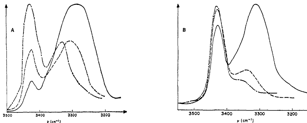
Figure 2. (A) t -BOC-Val 5 OMe: —, 2.55 \times 10^{-3} ; ---, 2.55 \times 10^{-4} ; -·-, 5.1 \times 10^{-5} . (B) t -BOC-Val 4 OMe: —, 9.23 \times 10^{-3} ; ---, 9.23 \times 10^{-4} ; -·-, 9.23 \times 10^{-5} . Concentrations in moles/liter.
