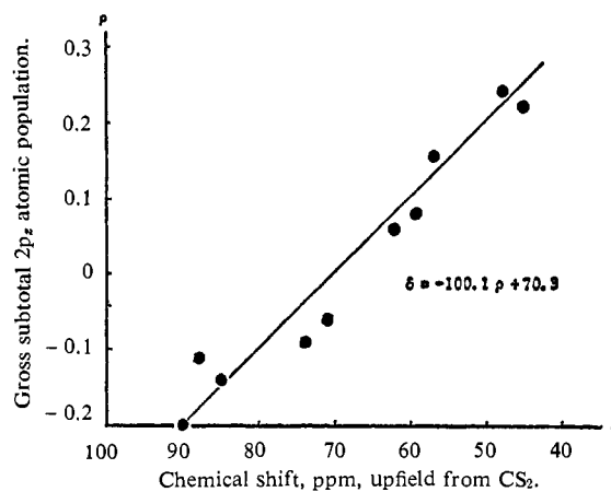
Figure 11. Correlation of calculated gross subtotal 2p_z atomic population with 13 C chemical shifts for the five-membered nitrogen heterocycles.
